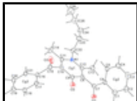
Fig. 1. The molecular structure of the title compound, showing the atom-numbering scheme. Displacement ellipsoids are drawn at the 30% probability.
