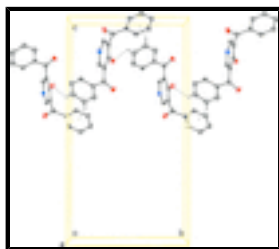
Fig. 2. A part of the crystal structure of the title compound showing the R_2^2(10) chain of rings along [010] generated by one C—H...O hydrogen bond and one C—H... \pi interaction.
